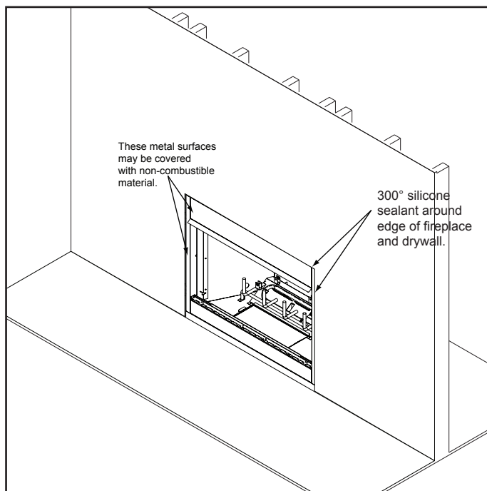
Figure 7.1 Non-combustible Facing
